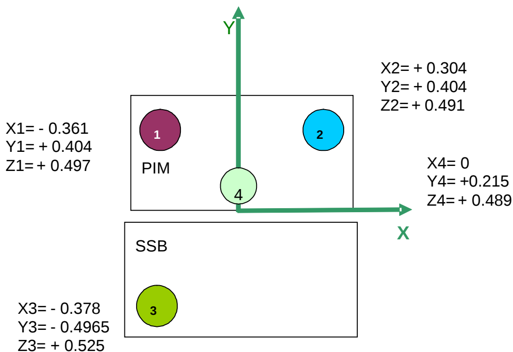
Figure 3 : Antennae mechanical positions in the PIM reference frame (in m)
